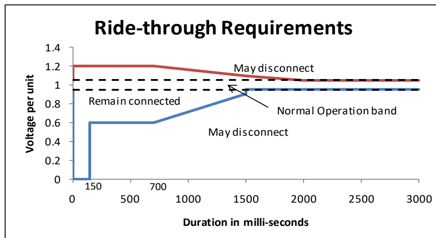
Figure 2 - Ride-through Requirements
